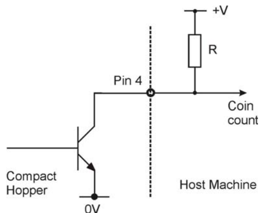
Figure 8: Opto Output Circuit
