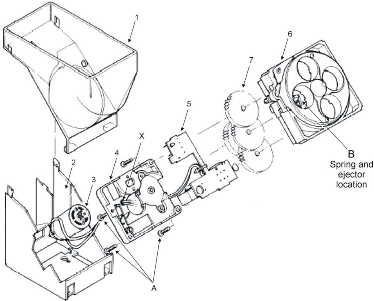
Figure 11: Exploded View
