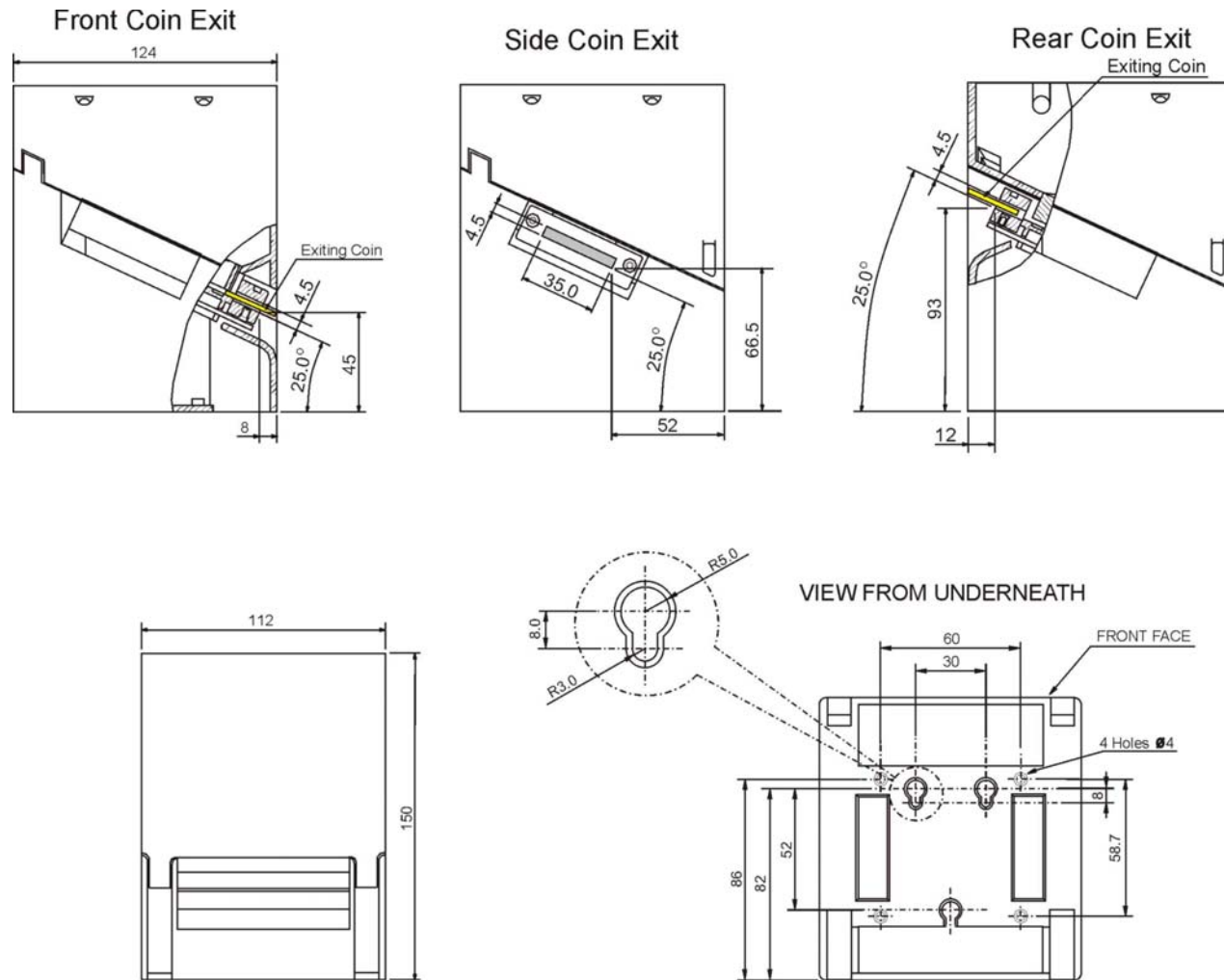
Figure 5: Square Bowl and Base (SBB) No Extensions, Hopper Dimensions
