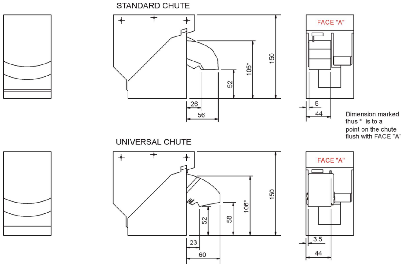
Figure 4: Standard Chute v Universal Chute Dimensions
